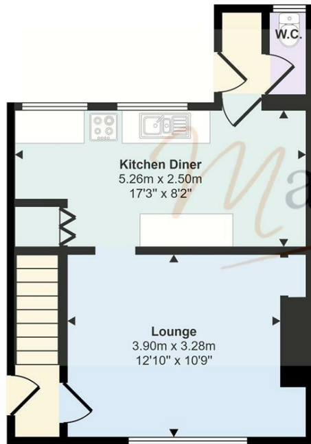
Ground Floor Approx 35 sq m / 376 sq ft
